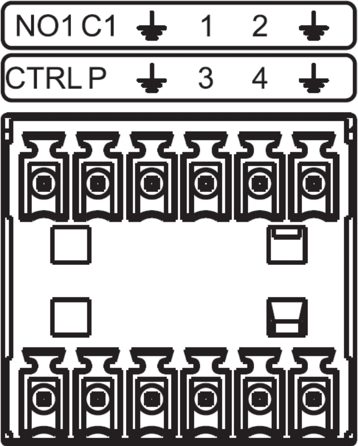
Alarm port description
