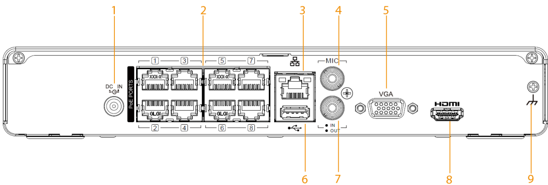
Rear panel (8-PoE port)
